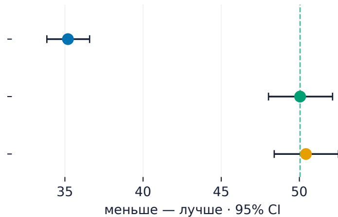
Conditional PPL
