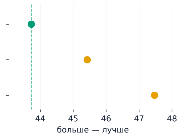
TruthfulQA MC2, %
