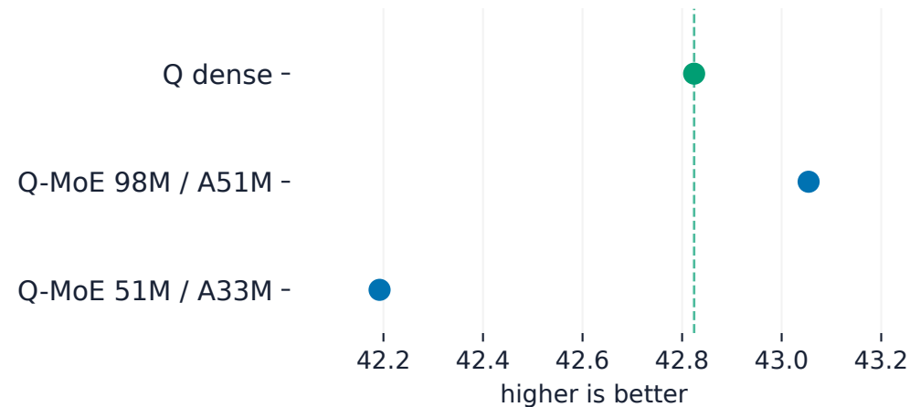
Task mean, %
