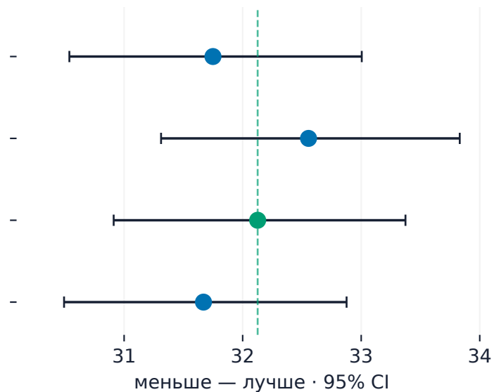
Conditional PPL · BF16
